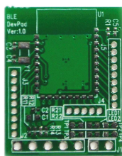
Bluetooth Module can be soldered on adapter PCB
